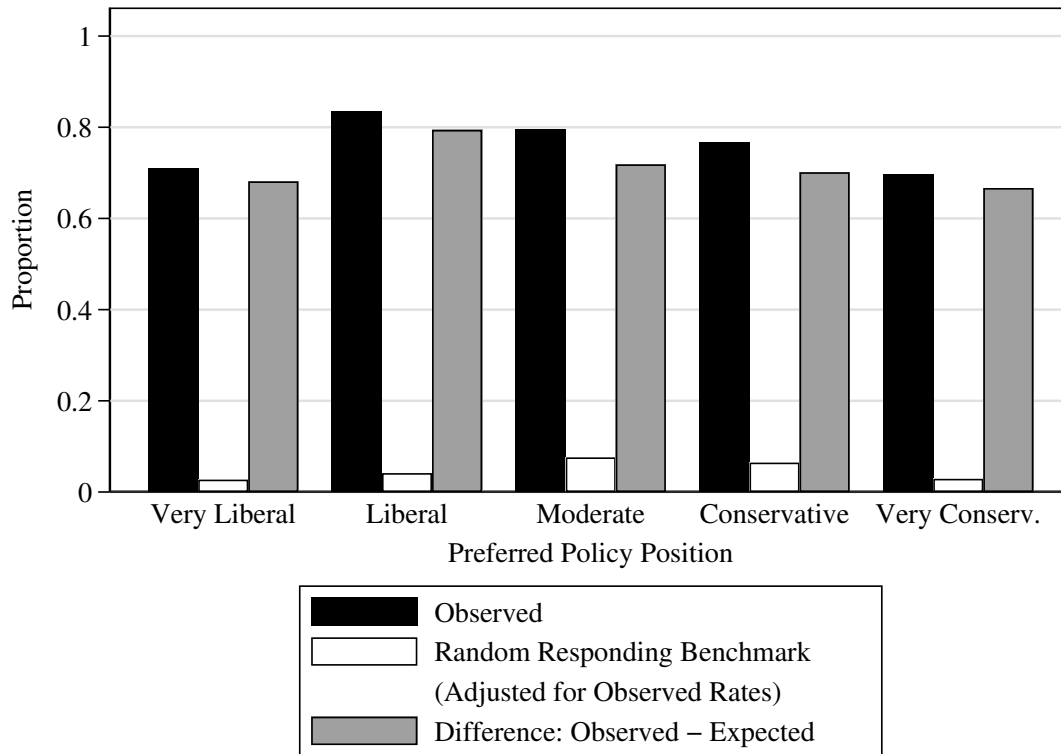
Figure C.2: Coherence in High-Salience Policy Domains, by Preferred Policy (Wave 2; N = 988 )
