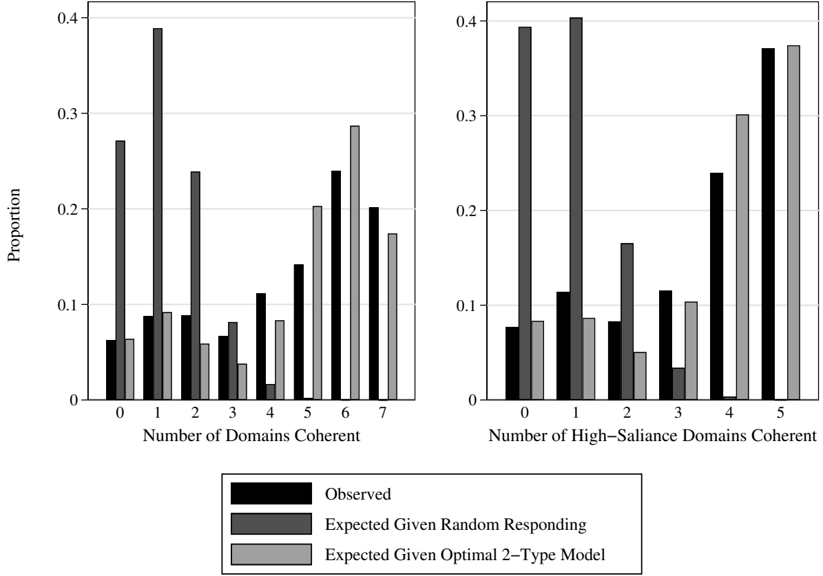
Figure C.4: Number of Issues Coherent: Weighted Wave 1 Data and Models
